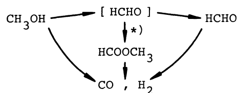
Fig. 1. Possible products in the dehydrogenation of methanol.
